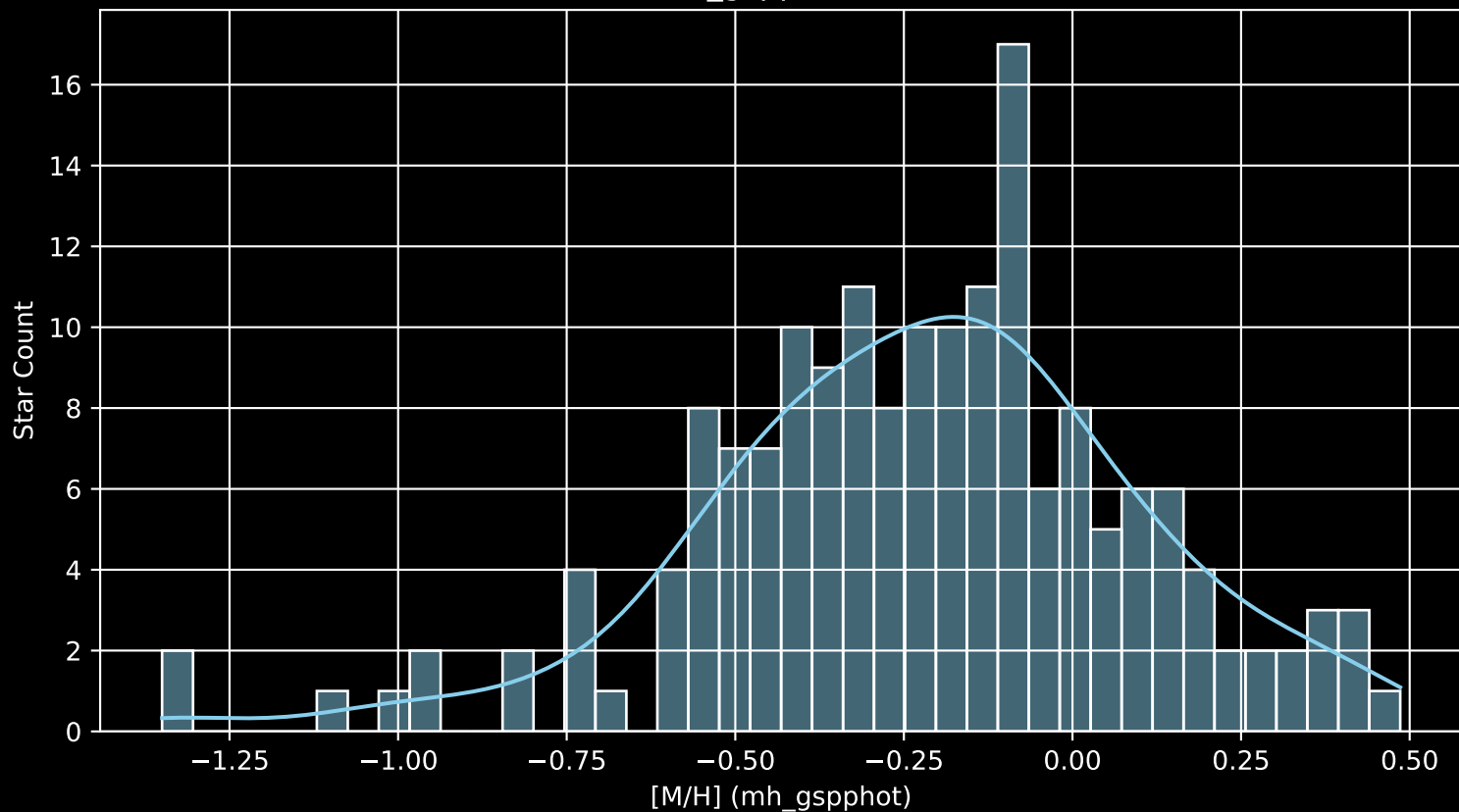
APOGEE DR17 Field: [264-26-O_TESS [M/H] (mh_gspphot) (n= 173)
