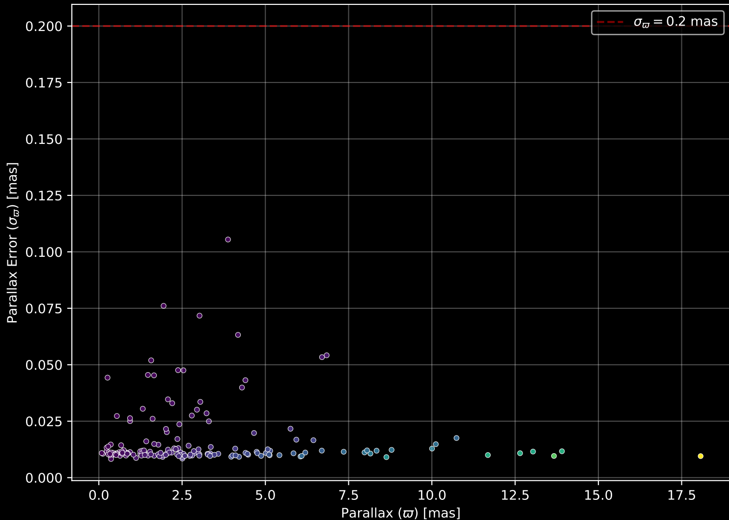
APOGEE DR17 Field: [264-26-O_TESS] Parallax Quality (n= 173)
