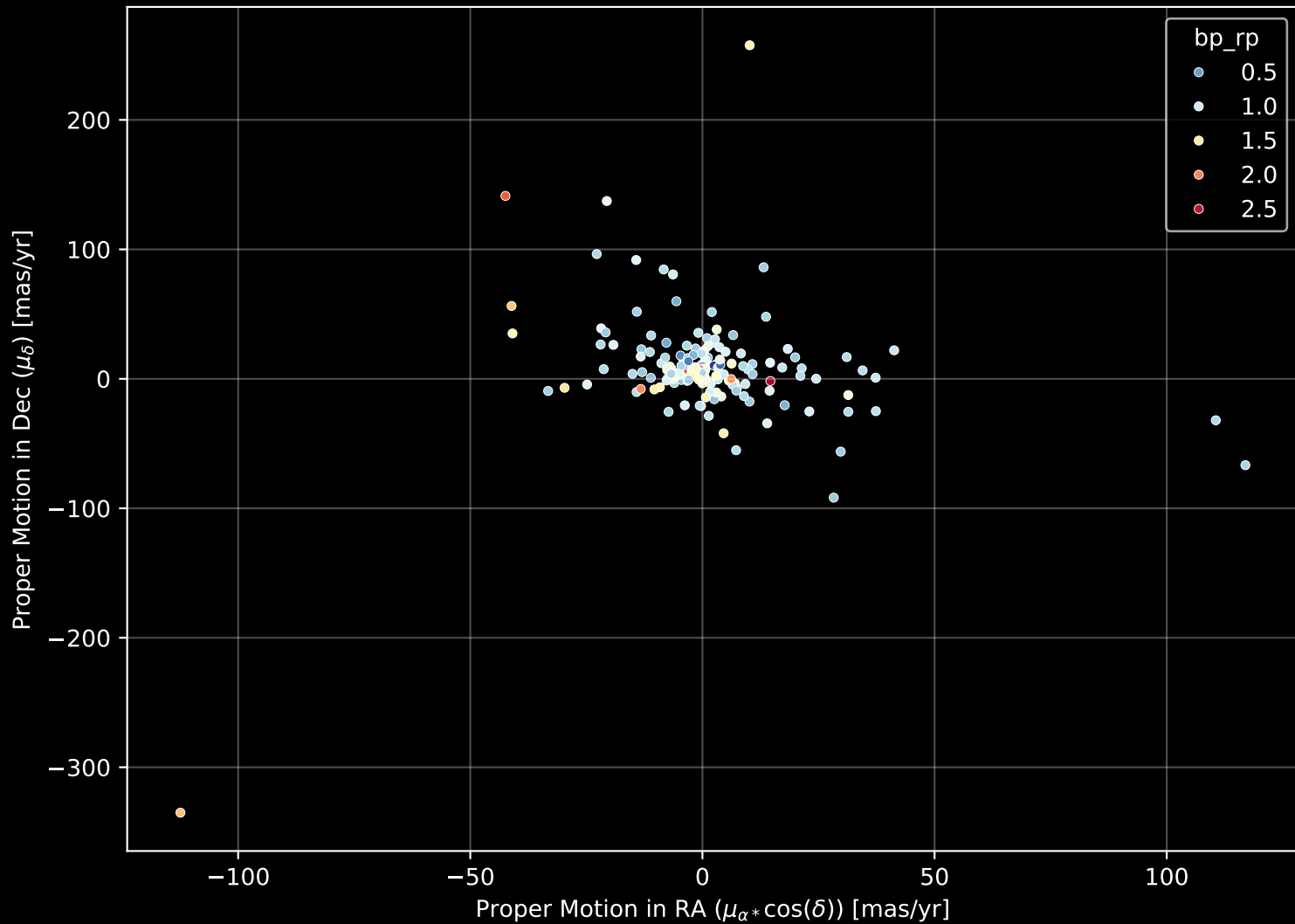
APOGEE DR17 Field: [264-26-O_TESS] Proper Motion Diagram (n= 173)
