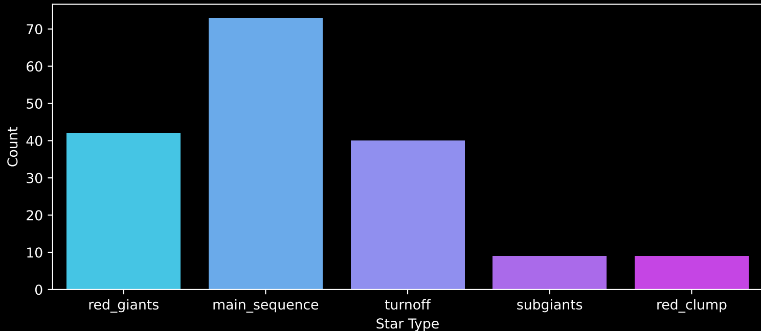
APOGEE DR17 Field: [264-26-O_TESS] Count plot of Star Type
