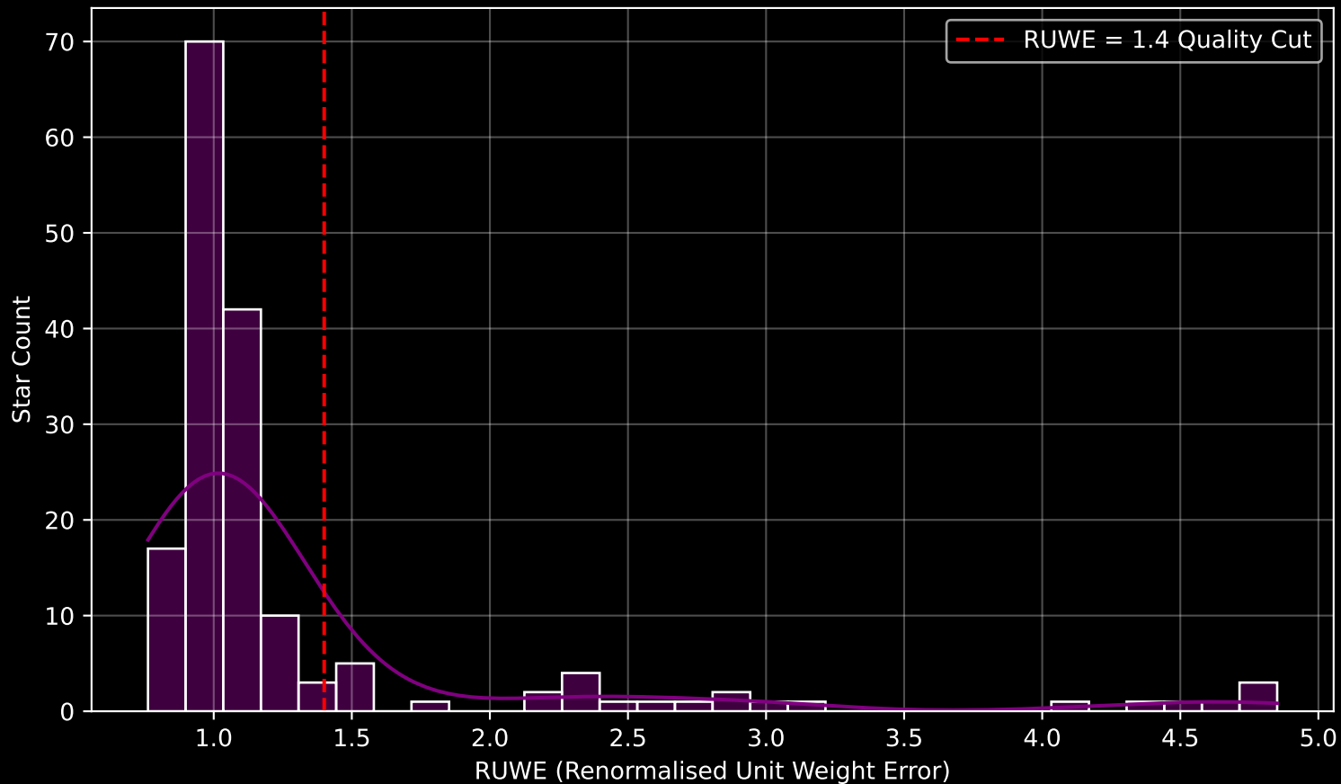
GAPOGEE DR17 Field [264-26-O_TESS] RUWE Distribution (n= 168)
